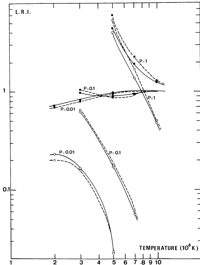
Fig. 12. Comparison of LRI's from cylinders and slabs, as functions of temperature. The pressures are indicated in \text{dyn cm}^{-2} . Open circles: cylinders observed at limb. Open squares: (vertical) slabs at limb. Full circles: cylinders on the disk. Full squares: (horizontal) slabs on the disk
