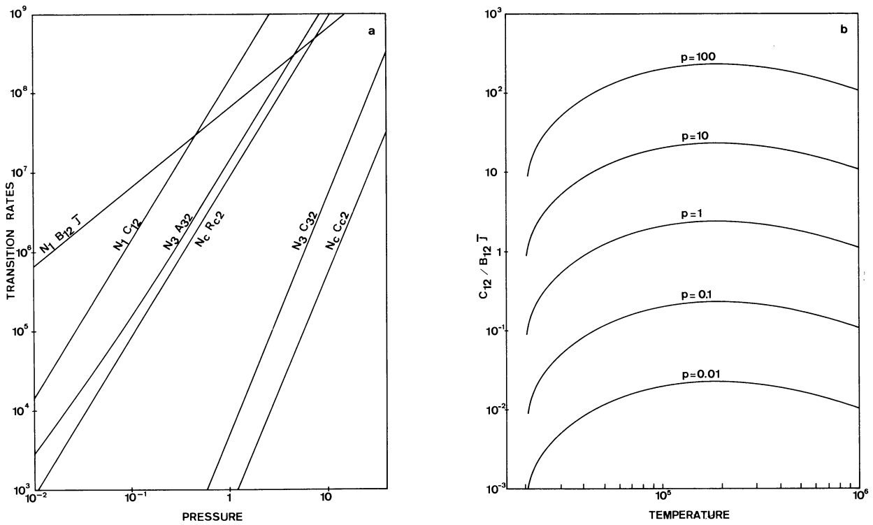
Fig. 1a and b. Comparison of efficiencies for different processes populating level 2 of the hydrogen atom. a Transition rates (in \text{cm}^{-3} \text{s}^{-1} ) as functions of pressure (in \text{dyn cm}^{-2} ) for a temperature of 10^5 \text{ K} . The curves are labeled with the corresponding mathematical symbols. b Ratio of collisional to radiative excitation rates for the (1–2) transition, as a function of temperature (in kelvins) for different pressures, indicated (in \text{dyn cm}^{-2} ) along the corresponding curves
