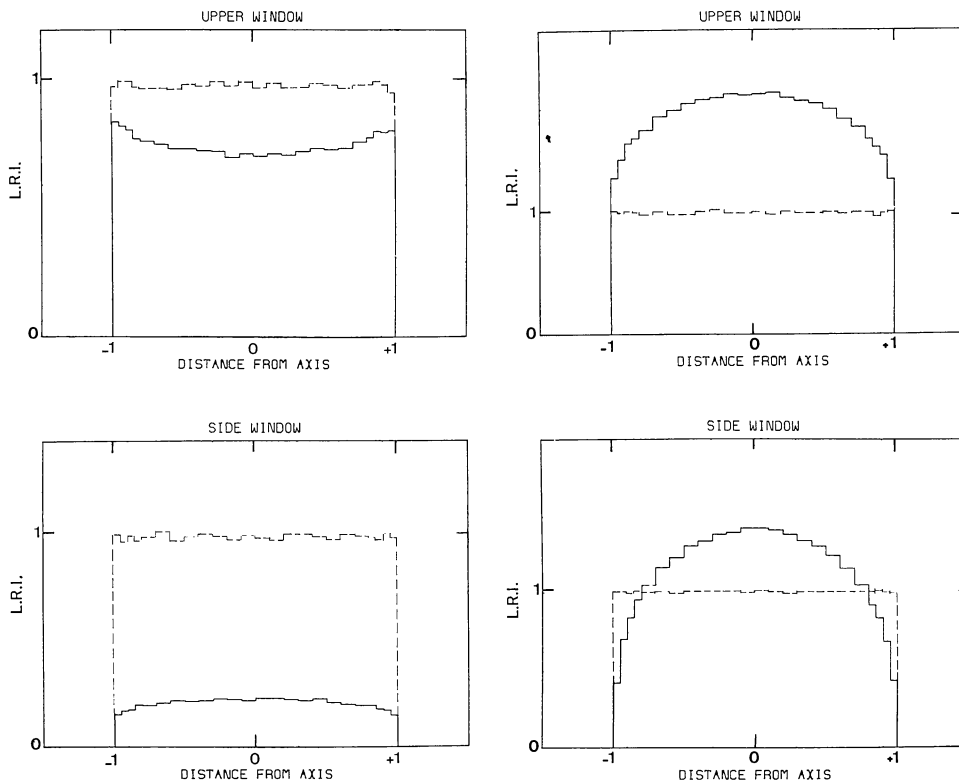
Fig. 10. Transversal variations of intensities (LRI) emitted by cylinders. Left: p = 0.01 \text{ dyn cm}^{-2} , T = 20000 \text{ K} . Right: p = 1 \text{ dyn cm}^{-2} , T = 70000 \text{ K} . Top: observation by the upper window. Bottom: observation by the side window. The distance from axis is in Mm. The solid lines represent the emission by the cylinder, and the dotted lines the solar disk's reference (constant except statistical noise)
