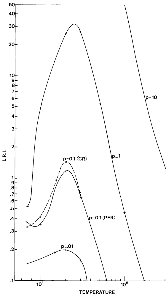
Fig. 7. Same as Fig. 5, but for vertical slabs
