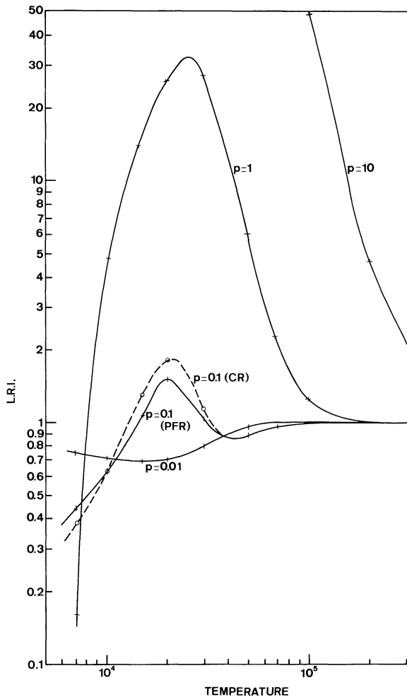
Fig. 5. Relative frequency-integrated intensities for horizontal plane-parallel slabs of thickness 1 Mm, as functions of temperature. Each curve corresponds to a constant pressure, which is indicated in \text{dyn cm}^{-2} . Solid curves refer to PFR computations in the Lyman lines. The dashed curve corresponds to the CR approximation
