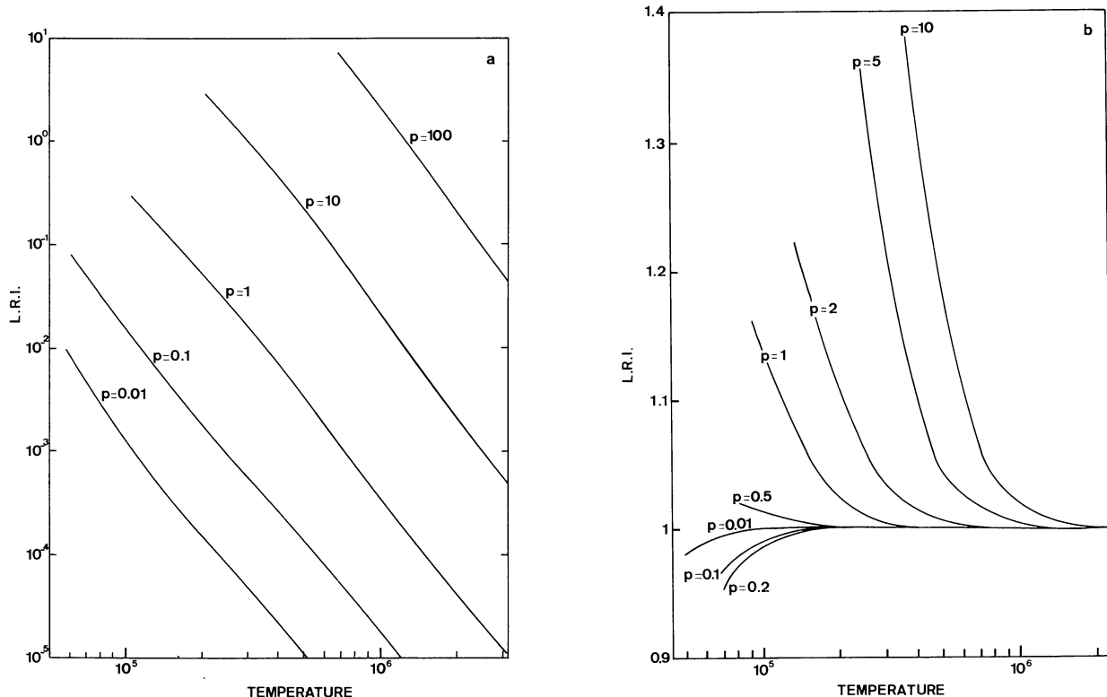
Fig. 4a and b. Optically thin objects: relative frequency-integrated intensities as functions of temperature (K) for a geometrical thickness of 1 Mm. a observations out of the limb, b observations on the disk. Each curve corresponds to a constant pressure, which is indicated in \text{dyn cm}^{-2}
