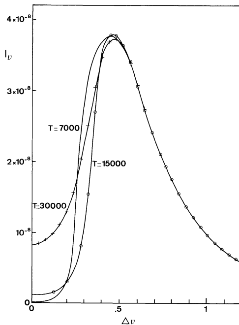
Fig. 6. Lyman- \alpha line profiles for horizontal slabs of thickness 1 Mm and pressure 0.01 \text{ dyn cm}^{-2} , observed at normal incidence. Each curve corresponds to a given temperature, indicated in K. Frequencies are in THz and intensities in \text{erg s}^{-1} \text{ cm}^{-2} \text{ sr}^{-1} \text{ Hz}^{-1}
