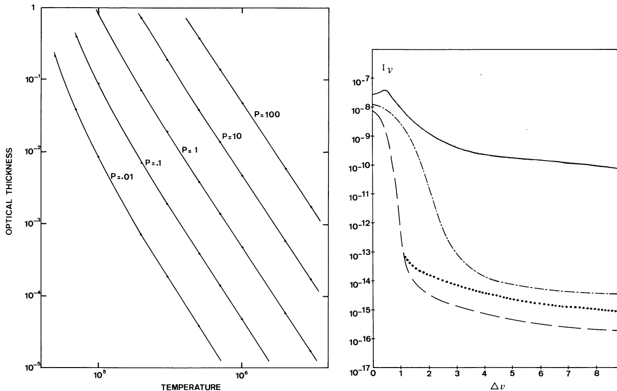
Fig. 2. Line center optical thickness as a function of temperature (in K) for different pressures (in \text{dyn cm}^{-2} , indicated along the curves), and a geometrical thickness of 1 Mm
