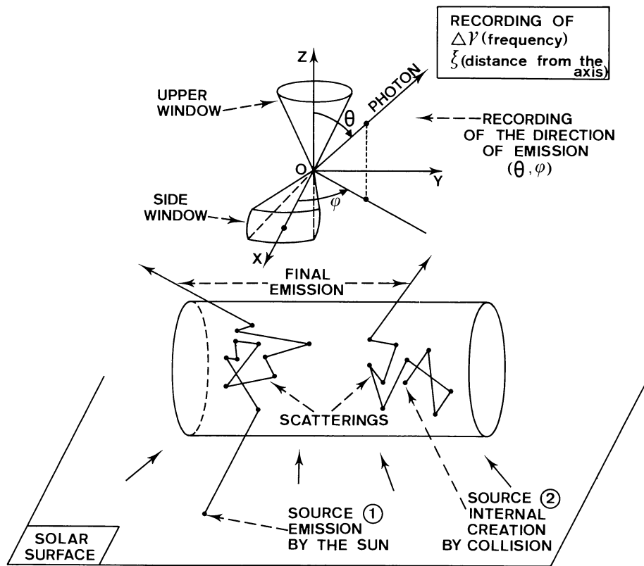
Fig. 8. Illustration of the Monte-Carlo method used for the computation of radiative transfer in cylindrical objects
