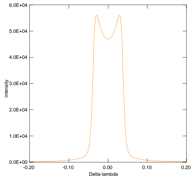
He II 304
