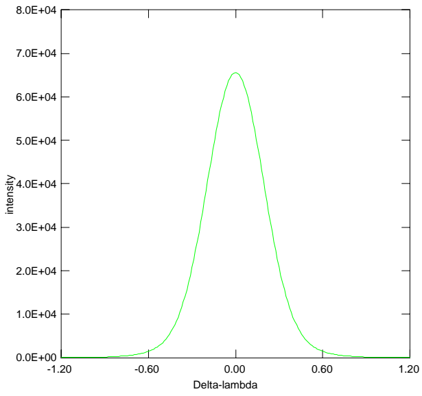
He I 10830
