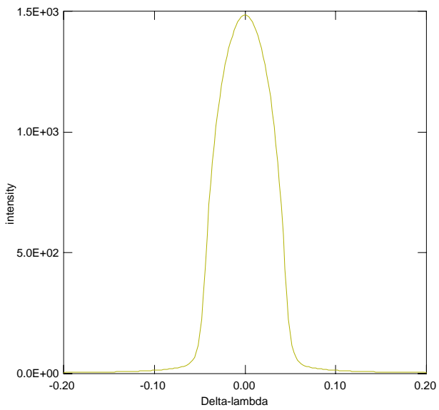
He I 537
