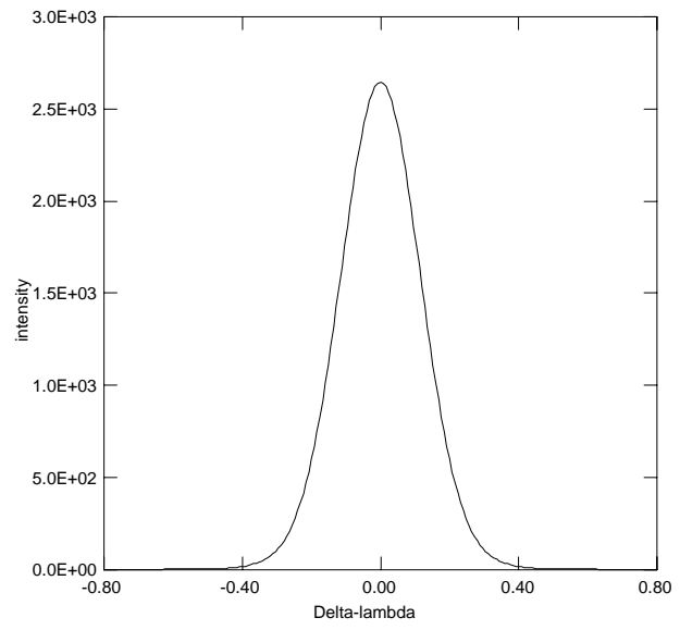
He I 6878
