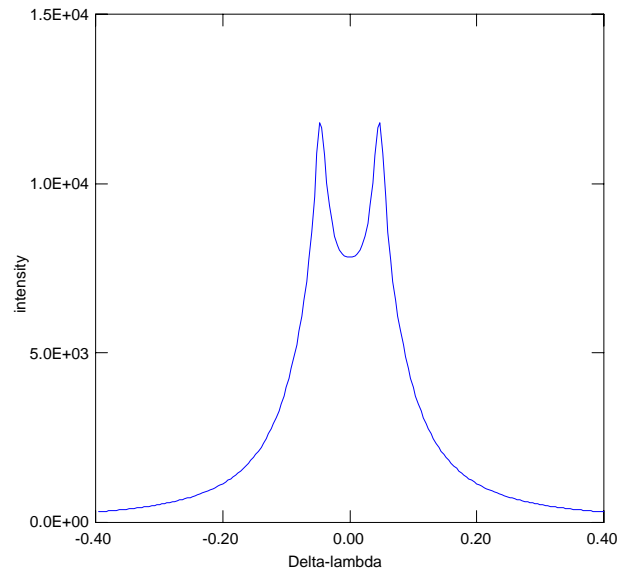
He I 584
