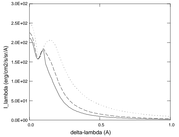
line 1 4 ( 972 A ), E = 1.36E+01
