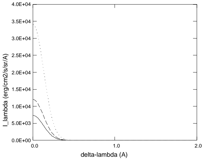
line 2 6 ( 4102 A ), E = 1.48E+03
