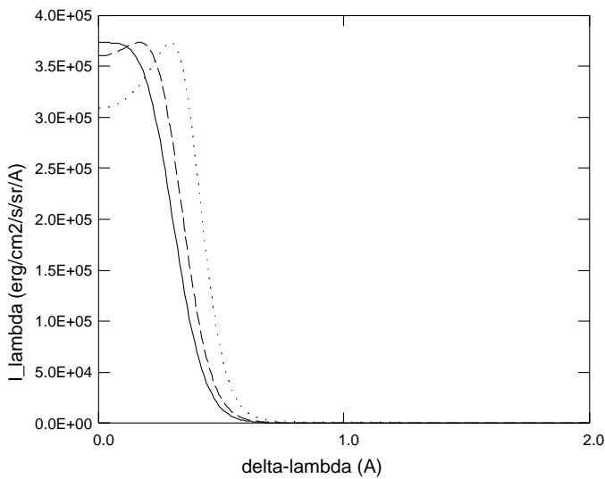
line 2 4 ( 4862 A ), E = 2.36E+05
