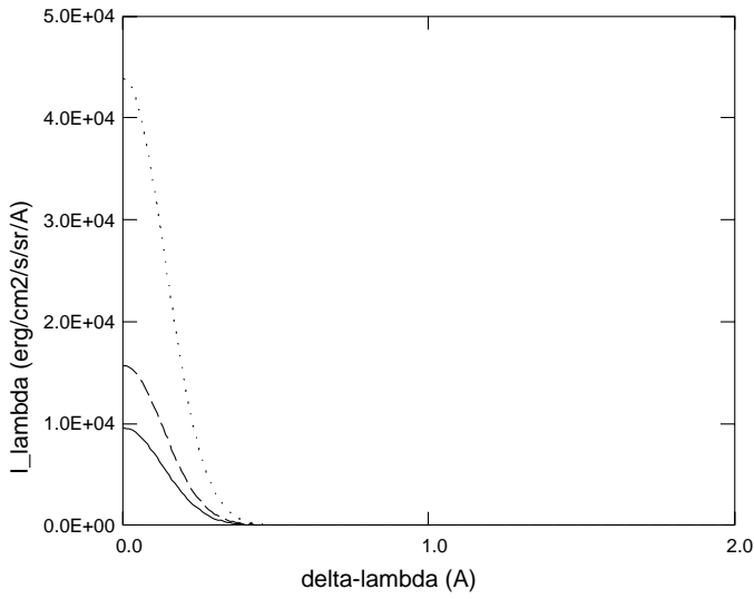
line 2 6 ( 4102 A ), E = 1.98E+03
