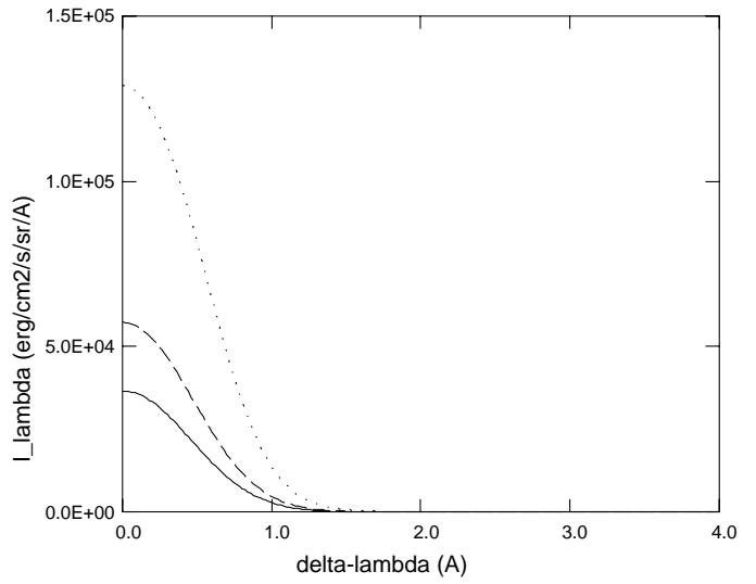
line 2 7 ( 3971 A ), E = 2.88E+04
