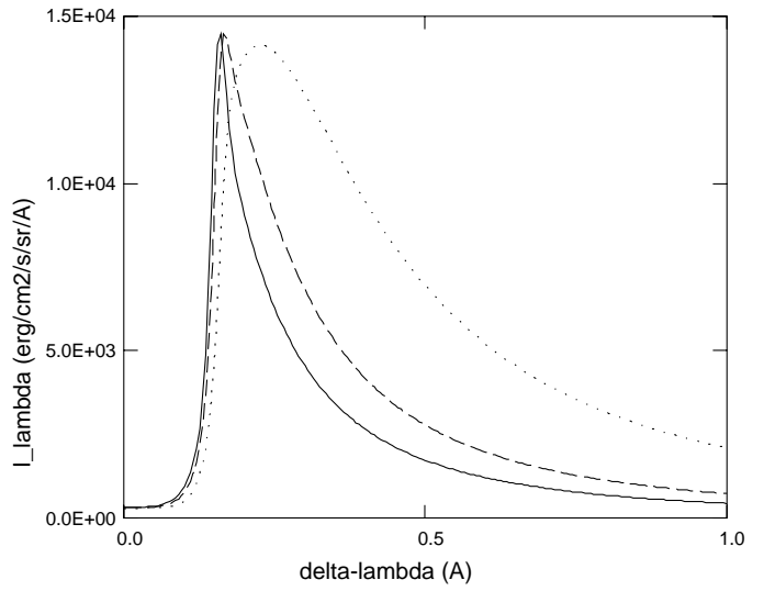
line 1 4 ( 972 A ), E = 5.85E+02
