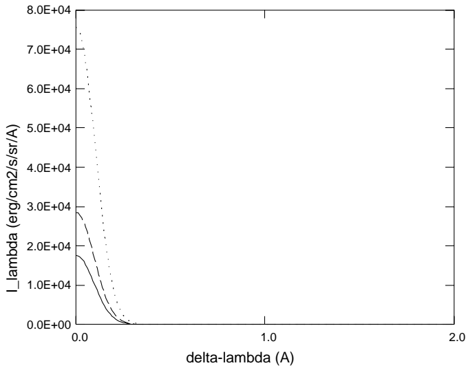
line 2 6 ( 4102 A ), E = 2.81E+03
