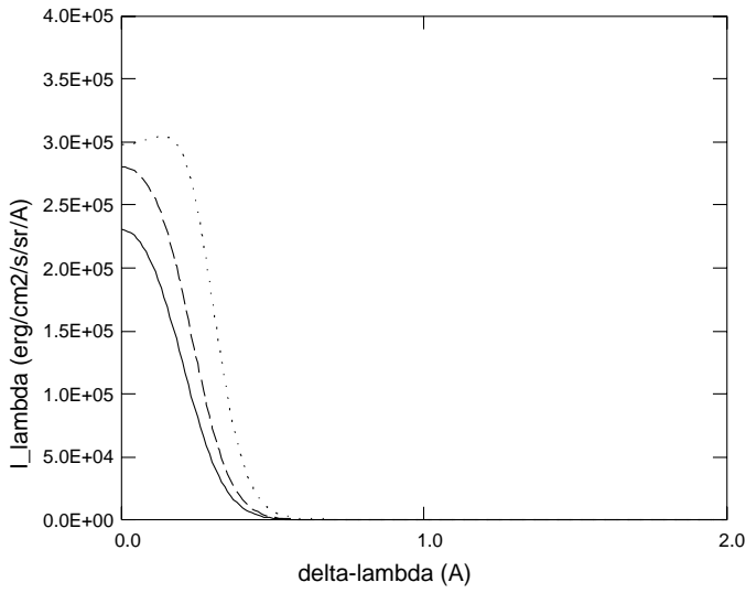
line 2 6 ( 4102 A ), E = 5.32E+04
