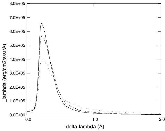
line 2 3 ( 6564 A ), E = 7.18E+05
