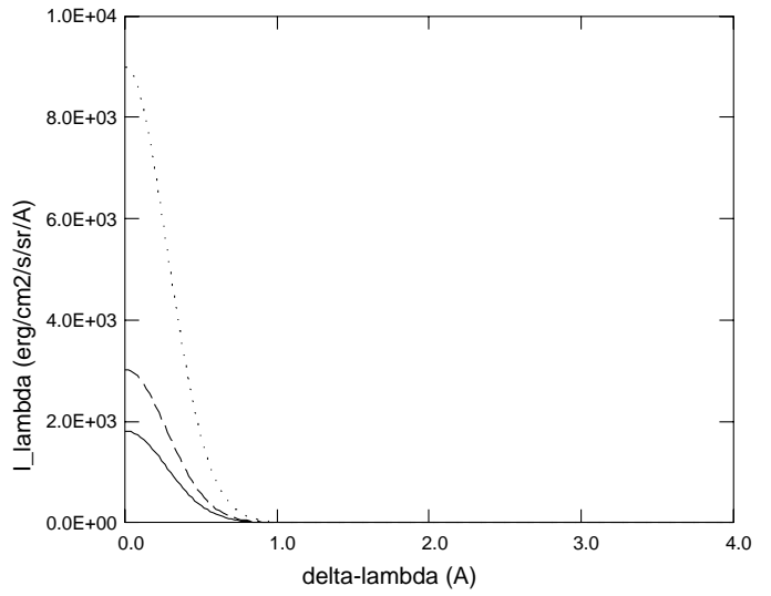
line 2 7 ( 3971 A ), E = 1.50E+03
