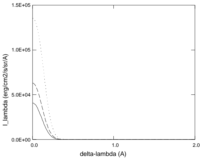
line 2 4 ( 4862 A ), E = 1.09E+04
