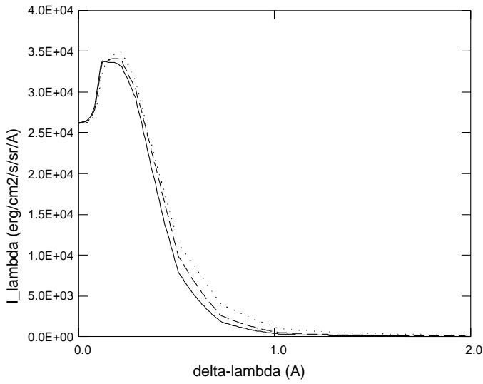
line 2 3 ( 6564 A ), E = 7.84E+04
