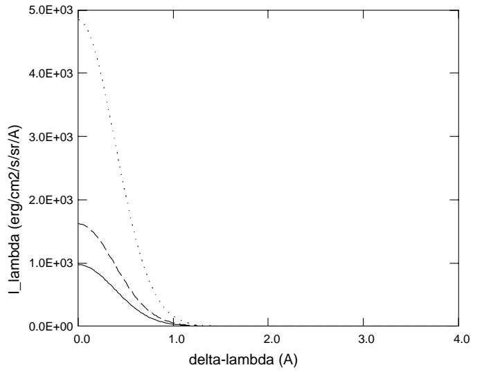
line 2 7 ( 3971 A ), E = 9.94E+02
