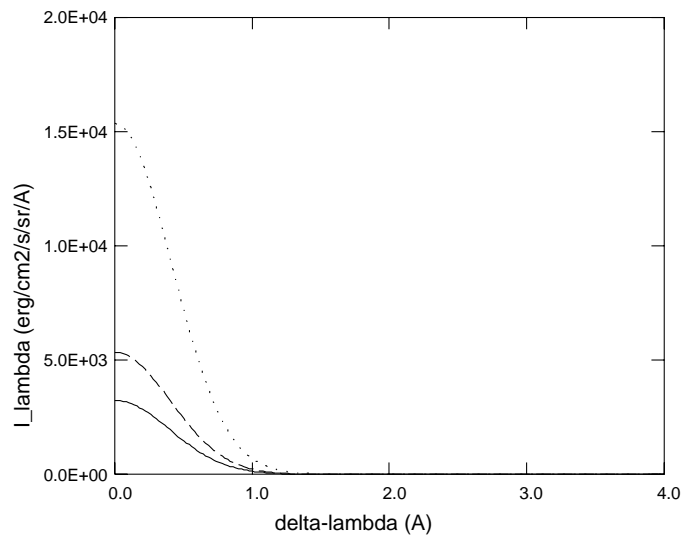
line 3 4 ( 18756 A ), E = 3.24E+03
