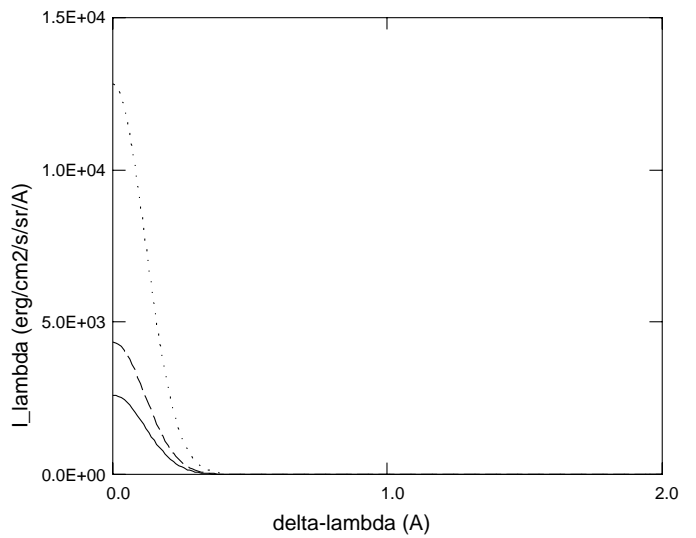
line 2 7 ( 3971 A ), E = 7.57E+02
