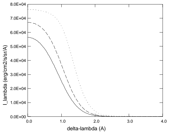
line 3 4 ( 18756 A ), E = 1.09E+05
