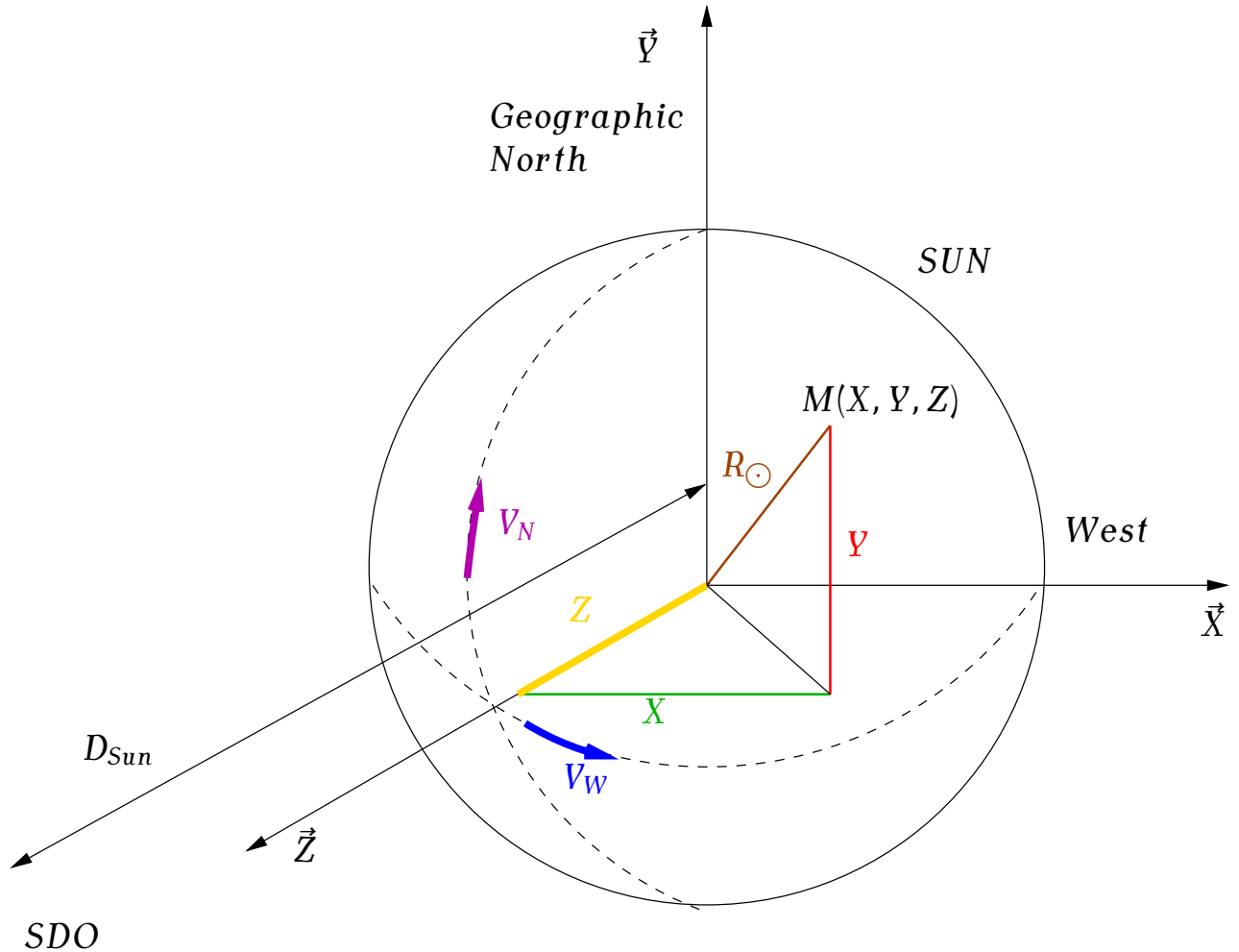
Figure 19: System of coordinates used in the computation of SDO motion correction parameters. The observer is on the satellite. Original HMI/SDO data have the North at the bottom and East on the right of the image; the images are rotated in order to have the North on top and East on the left.
