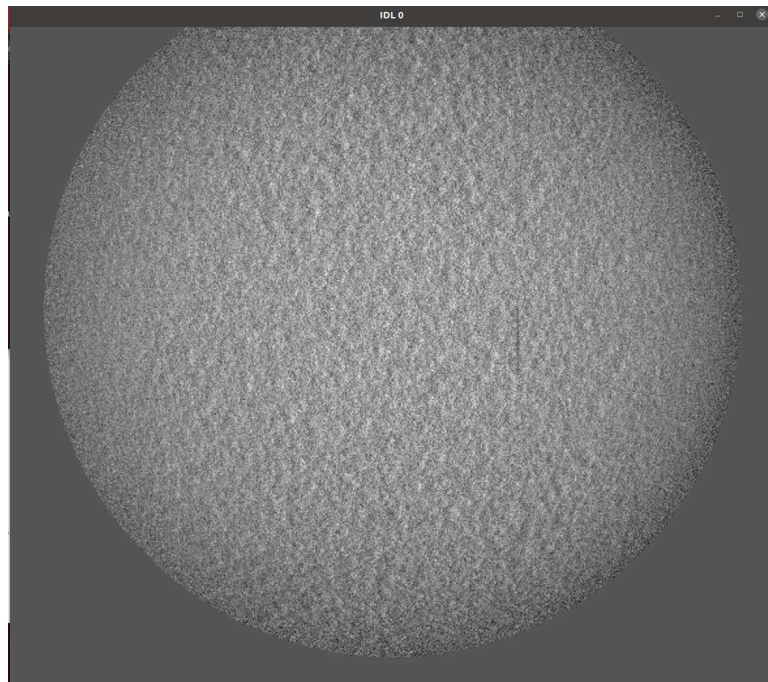
Figure 23: Solar granules close to the limb - observations on November 29, 2018
