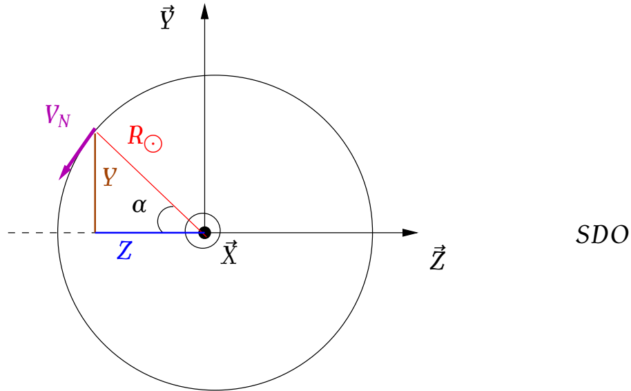
Figure 20: System of coordinates used in the computation of SDO motion correction parameters. The observer is on the satellite.
