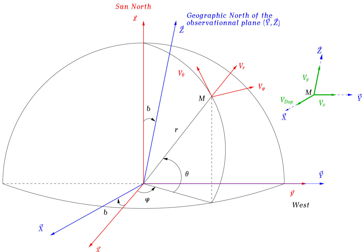
Figure 21: Coordinate system used in formulas : velocity components (V_x, V_y, V_{Dop}) at point M in observation reference (\vec{X}, \vec{Y}, \vec{Z}) and velocity components (V_r, V_\theta, V_\varphi) at point M in Sun reference (\vec{x}, \vec{y}, \vec{z}) .
