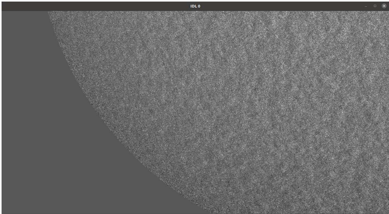
Figure 24: Solar granules close to the limb - observations on November 29, 2018
